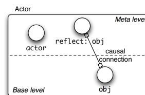
Figure 1. Layout of an AmbientTalk actor.
