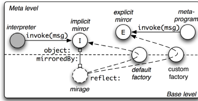
Figure 2. Implicit versus Explicit Mirrors
