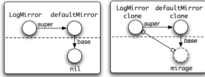
Figure 3. Left: an unabsorbed mirror prototype. Right: an absorbed mirror instance causally connected to a mirage.
